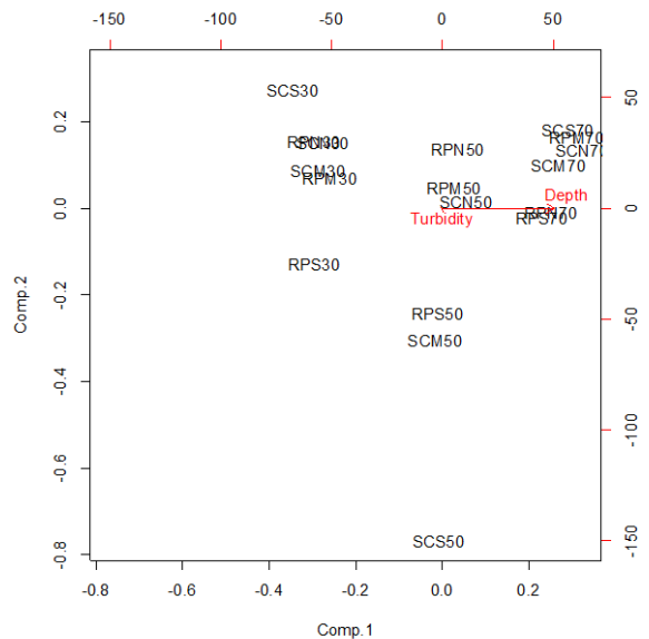
Figure 6: Principle Components analysis of water properties of tow stations
