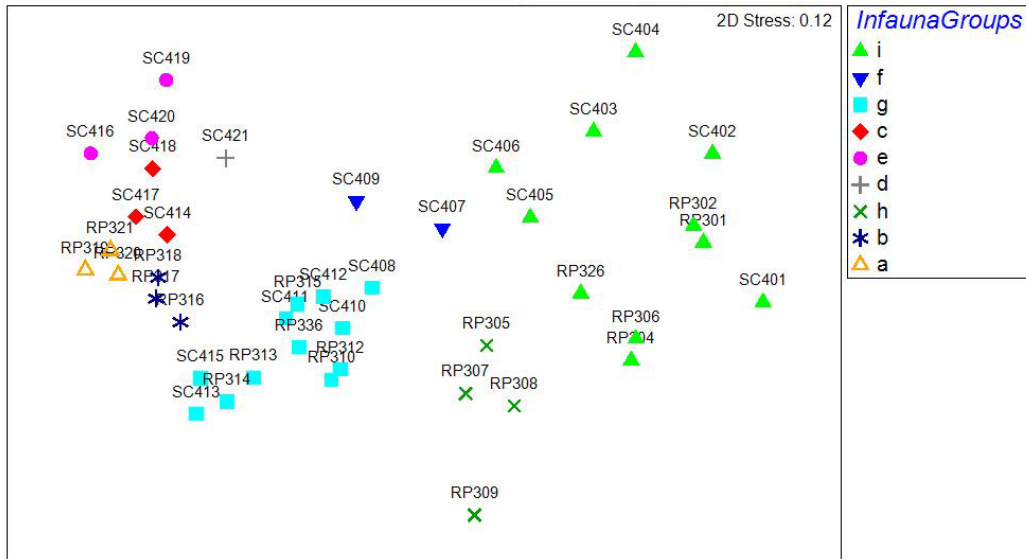
Figure 5: Multi-dimensional Scaling plot of similarity in infaunal invertebrate assemblages among trawls. Data were square root transformed. Significant clusters were determined used Bray Curtis similarity. Stations with the same symbol are statistically indistinguishable.
