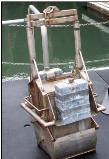
Figure 2: Box corer used for collecting infaunal invertebrates.
