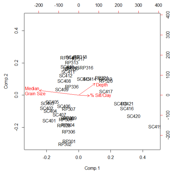
Figure 4: Principle Components Analysis of physical attributes of box core samples.
